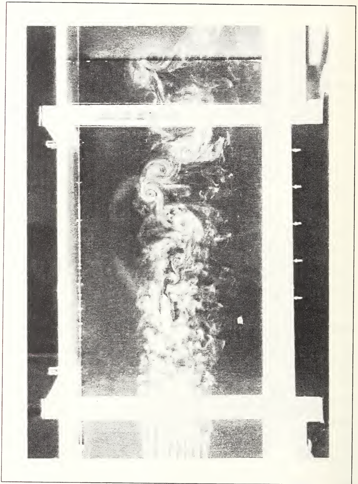
Figure 4.6 K_p = 1.8008 , h/2b = .1977 , 1.56 ft/s
